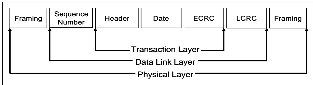
Figure 2-2. Packet Flow through the Layers
