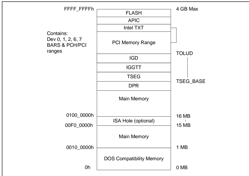
Figure 2-3. Main Memory Address Range
